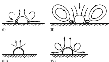
Fig. 3. Microstreaming pattern near a pulsating hemisphere bubble trapped at a plate wall (Elder, 1959).
